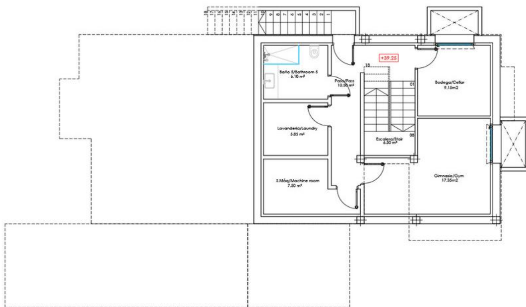
BASEMENT FLOOR
